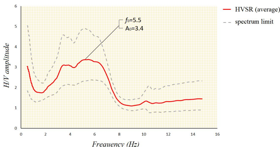
Figure 1. Amplitude and frequency coupling spectrum in seismometric data measured in a quiet state
