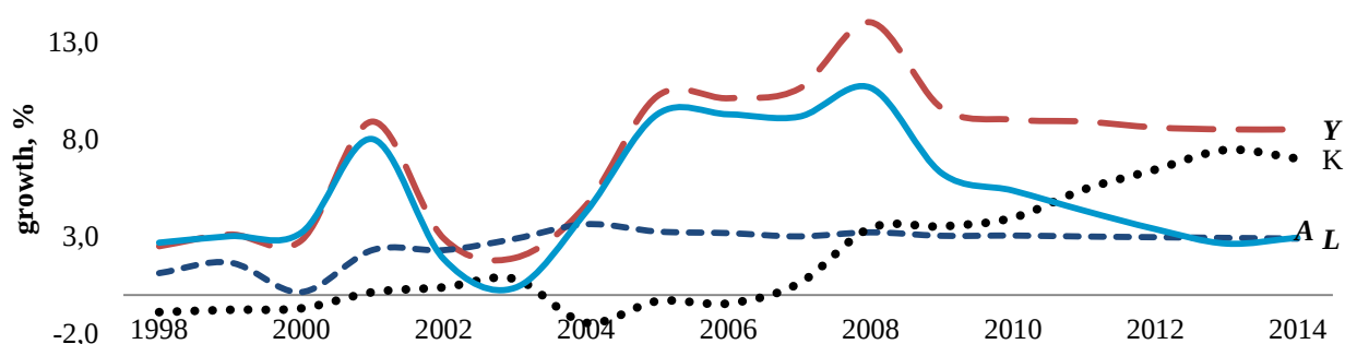
Figure 2. The parameters of the production function of a small city.
